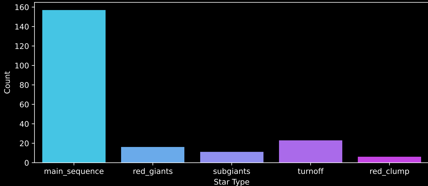
APOGEE DR17 Field: [K2_C1_255+56_btx] Count plot of Star Type
